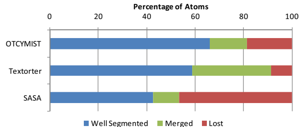
Figure 2. Atom-based Segmentation Results as per [12]
