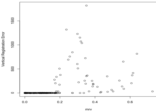
Figure 8. Relation between m_{rv} (x axis) and the vertical registration error (y axis). Accurate registrations (vertical error close to 0) have a m_{rv} value lower than 0.19. When m_{rv} is higher, we can not guaranty a pixel accurate registration.
