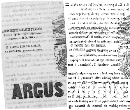
Figure 4. Results of the de-skew algorithm based on the extracted bleed-through and noise pixels : on the left the original document, on the right the de-skewed document (only the extracted bleed-through pixels are used).
